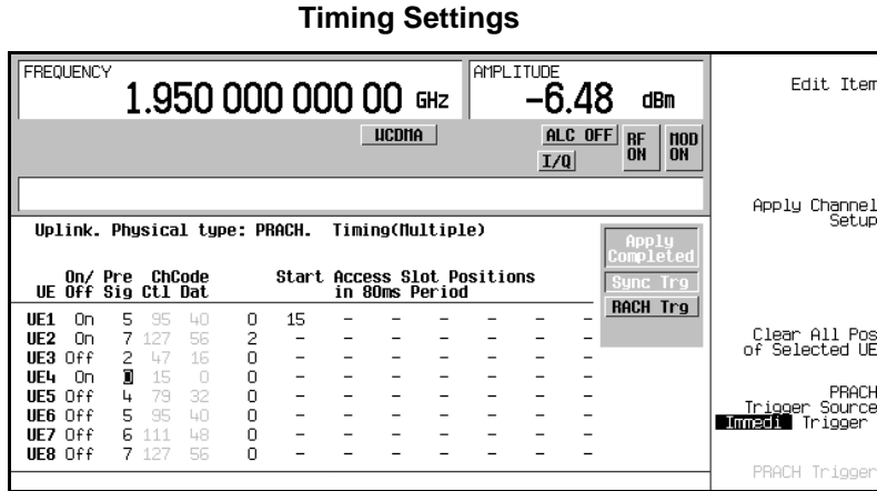
Figure 16-32 Multiple PRACH Timing Setup
