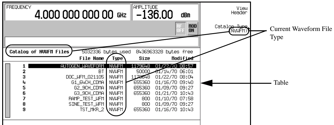
Figure 4-9 NVWFM Waveform Files Showing
